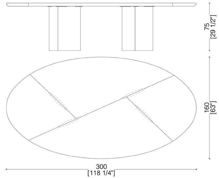
D 60 B2 Elliptical table
