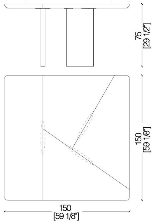
BD 60 D Square table
