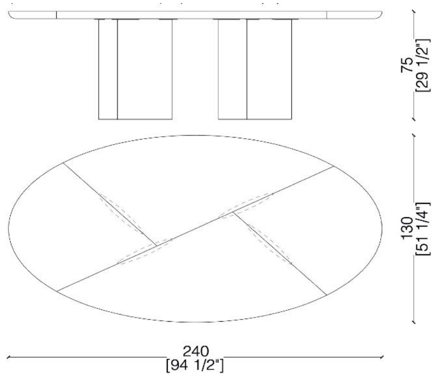
BD 60 B Elliptical table
