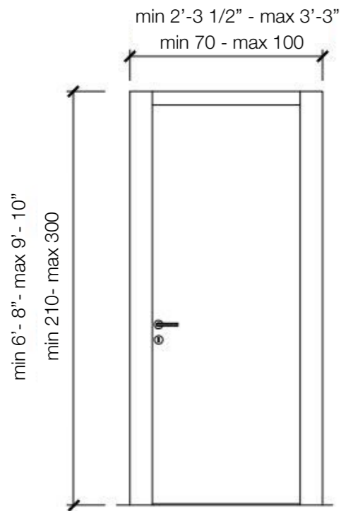
Single Hinged Door
